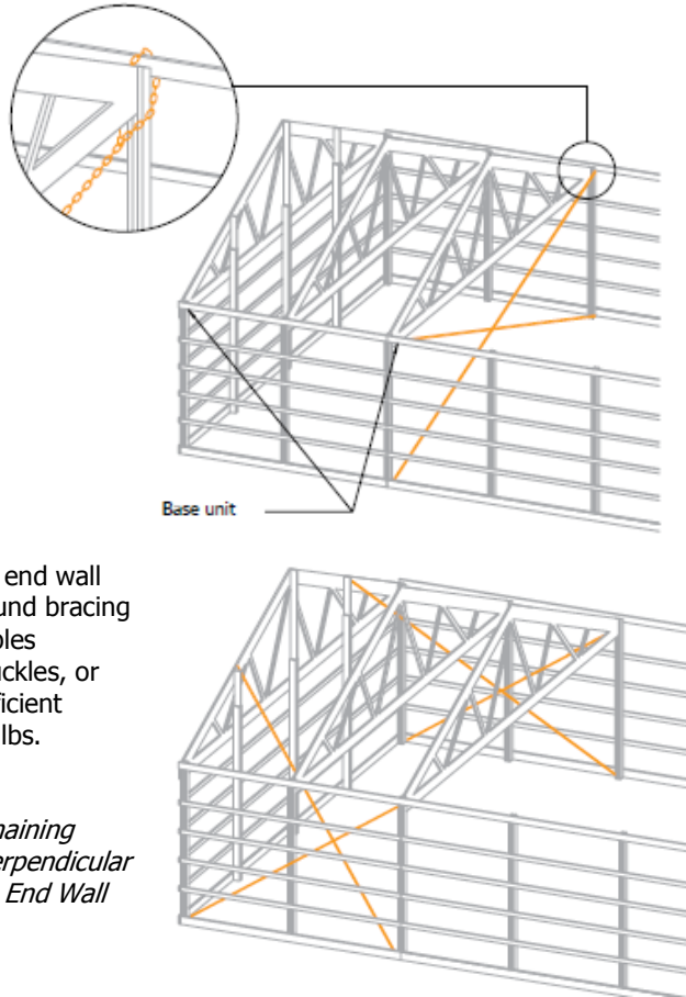
Column – Truss Bracing Parallel
