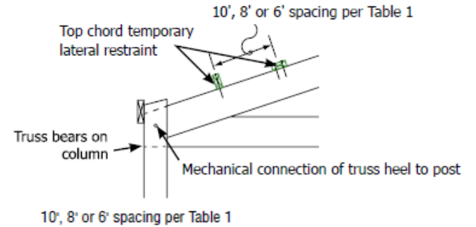
Mechanical Connection at Heel and Top Chord Temporary Lateral Restraint
